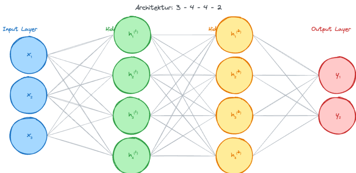
Figure 2: neuronales_netz.excalidraw.png
